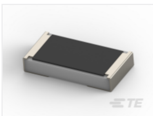
TE Part #2176469-2 TLRP 2010 2.0W R020 1% 75PPM 4K RL
