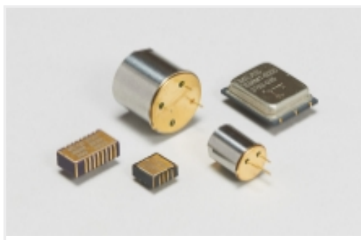
Piezoelectric Accelerometers(2)
