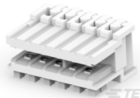
TE Part #2-284932-5 DUOPLUG STD FEMALE CONN., 5 POS.
