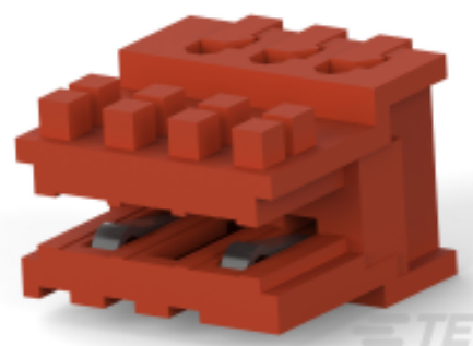
TE Part #4-284931-3 DUOPLUG Standard, female conn.
