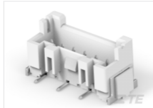
TE Part #2365497-6 EP2.5 single row SMT header, GWT, 6P
