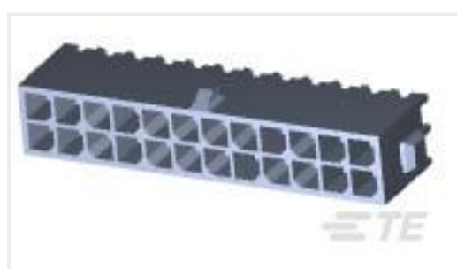
TE Part #5-794632-4 24P MICRO MNL ASSY,VRT,HDR,LF
