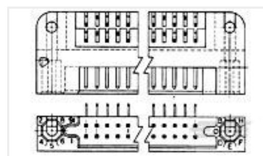
TE Part #531720-9 2 ROW BOX PIN 90 POS R/A
