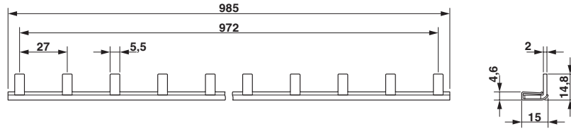
Dimensional drawing
