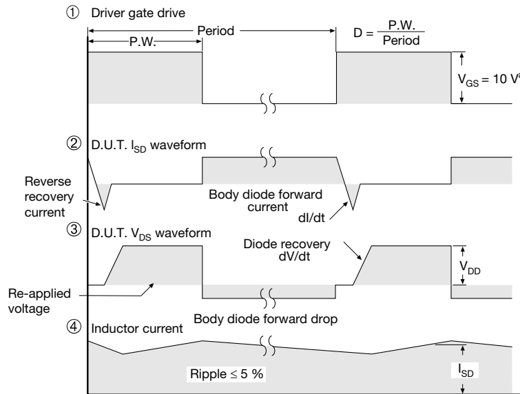
Fig. 11 - For N-Channel
