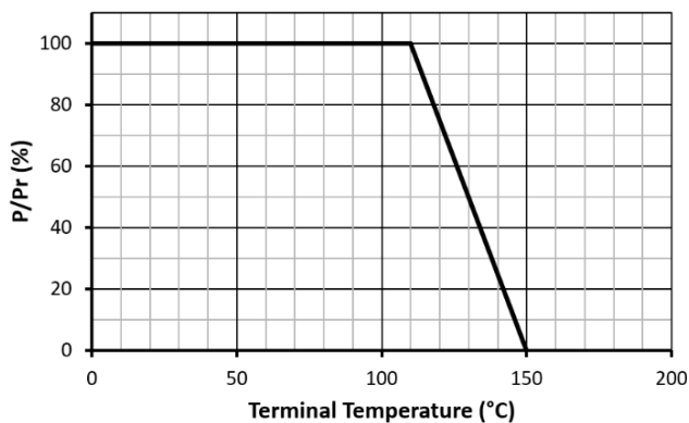
Temperature Derating
