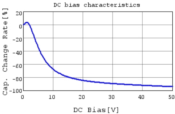
GRM155R61H224KE01 C-DC bias capchange, 25.0c
