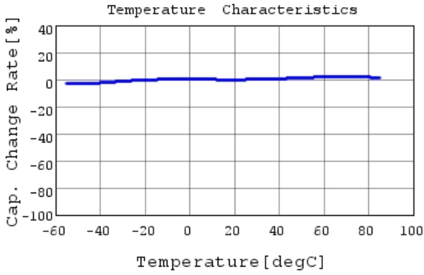
GRM155R61H224KE01 C-Temp. capchange, DC0.0V,
