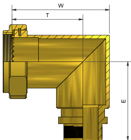
90° BACKSHELL - TYPE 1
