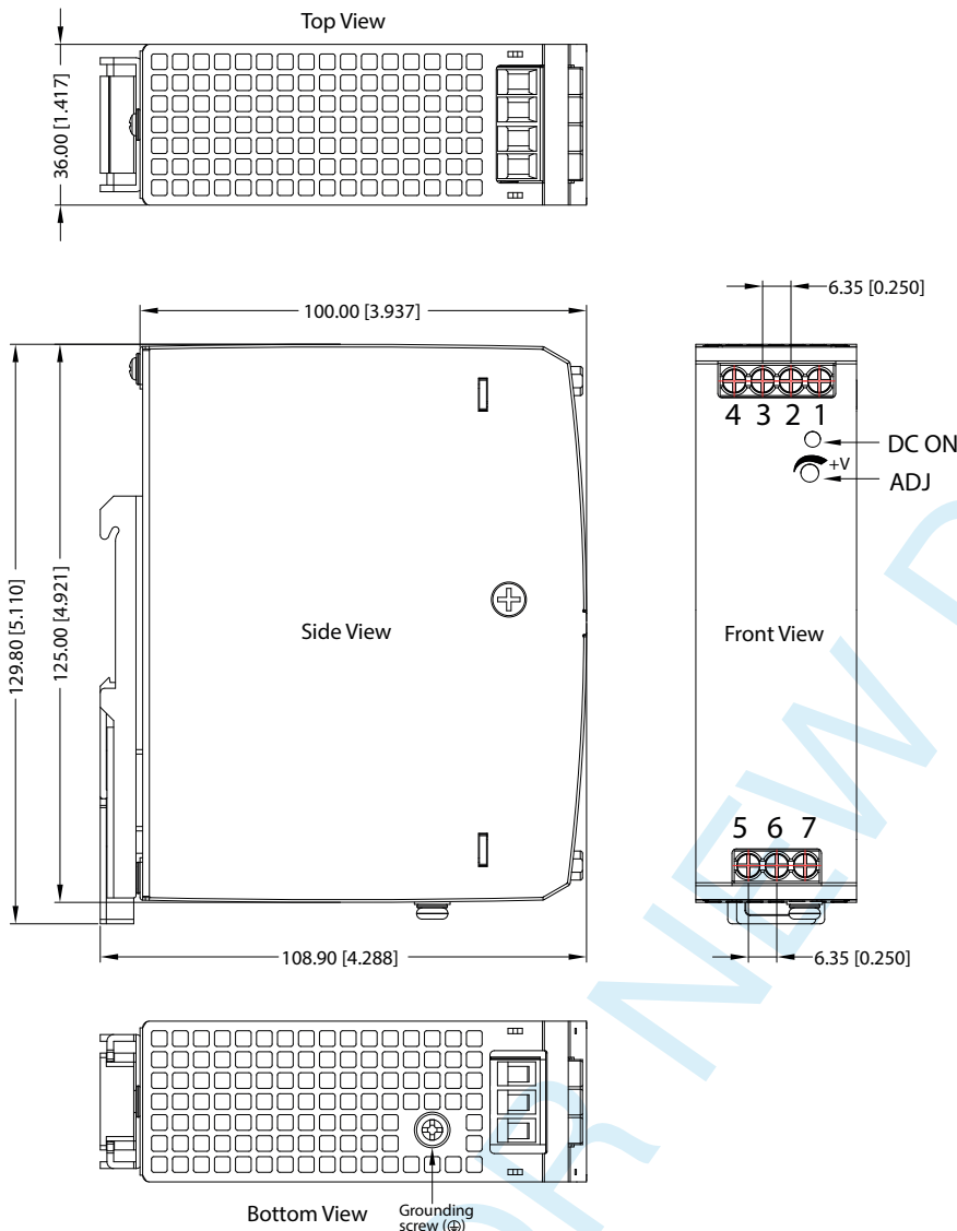
Figure 5. Mechanical Drawing
