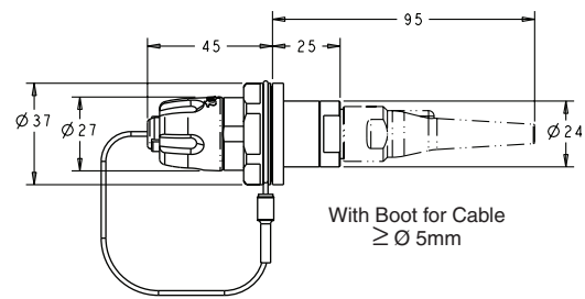
PRO BEAM Jr. Standard Bulkhead Connector, with Boot
