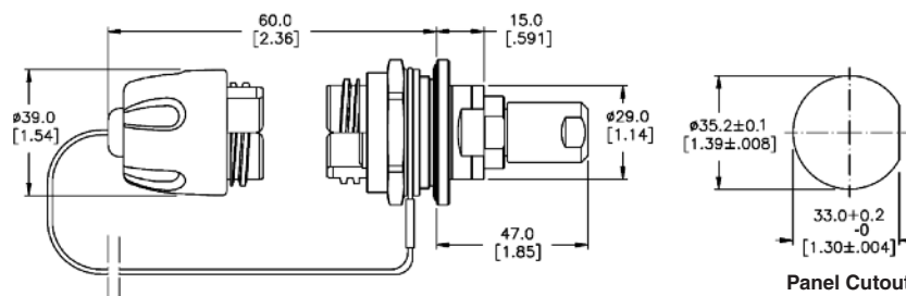
PRO BEAM Sr. D-Hole Bulkhead Connector with Standard Cable Adapter
