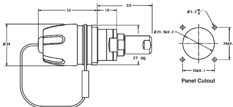
PRO BEAM Sr. Square Flange Mount Bulkhead Connector with Standard Cable Adapter
