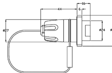
PRO BEAM Jr., Low Profile, Square Flange Mount Bulkhead Connector
