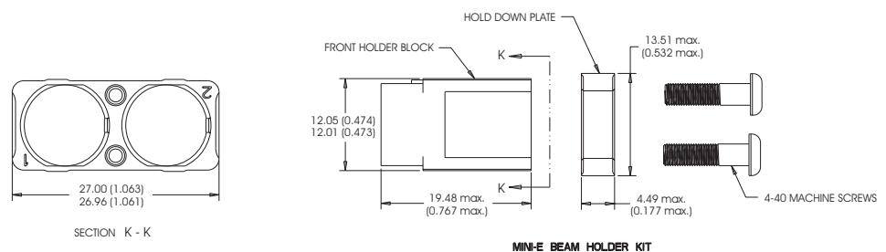
MINI-E BEAM HOLDER KIT
