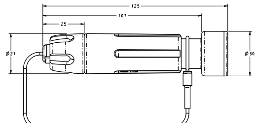
PRO BEAM Jr., Loopback Plug Connector
