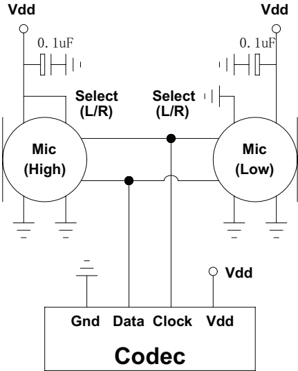
Dual Microphone
