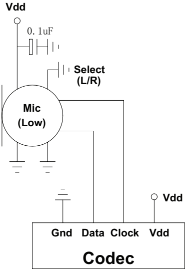
Single Microphone
