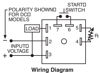
Wiring Diagram
