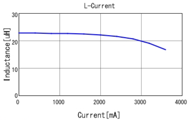
#B952AS-H-220M=P3 L-Current 20degC
