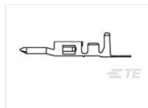
TE Part #2238016-1 VAL-U-LOK PIN BR SN 18-22AWG
