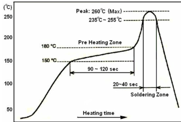
Max Soldering Time: 3 times Temperature profile for evaluation
