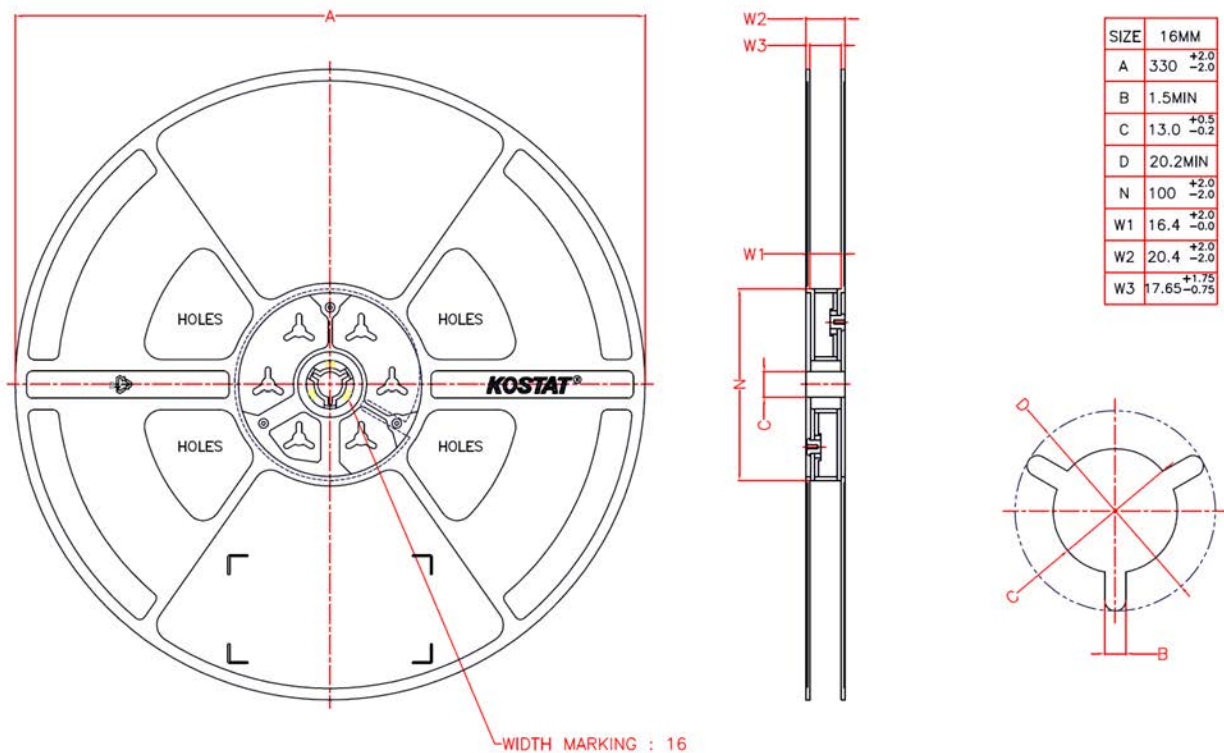
Figure 10.2. Reel Dimensions
