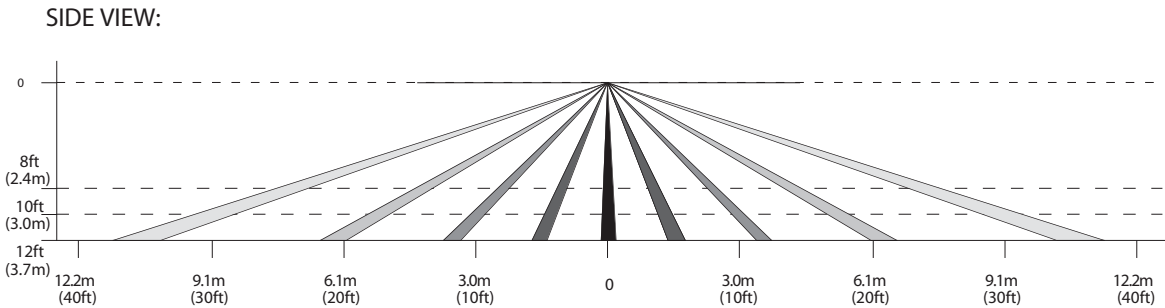
Figure 3. CM 0.77 GI V2 Lens Specification: Floor Coverage, Side View
