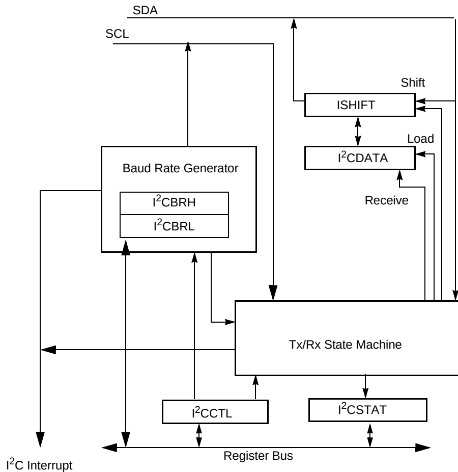
Figure 26. I²C Controller Block Diagram
