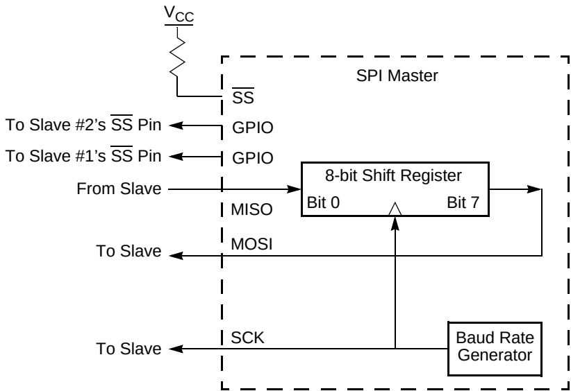
Figure 22. SPI Configured as a Master in a Single-Master, Multiple-Slave System
