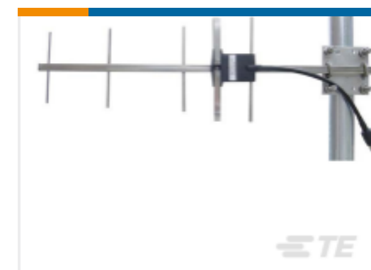
TE Part #YA9-9 YAGI,860-960MHz 5,9dBi
