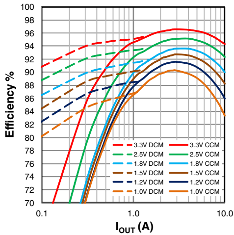
Figure 19: Efficiency, V_{IN}=5V
