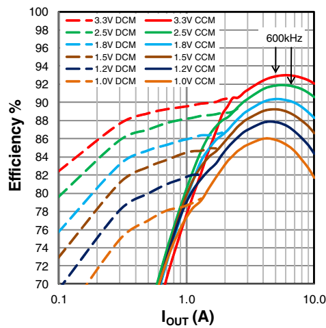
Figure 21: Efficiency, V_{IN}=12V
