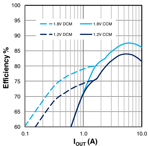
Figure 23: Efficiency, V_{IN}=19.6V
