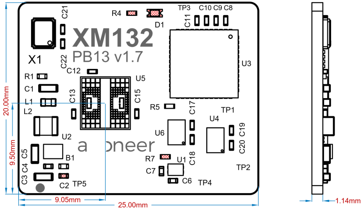
Figure 5.1. Component placement top and side views.
