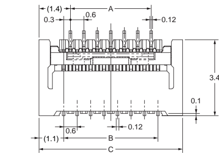
Cross-section diagram: X-X
