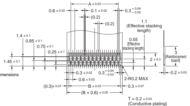
Applicable FPC Dimensions
