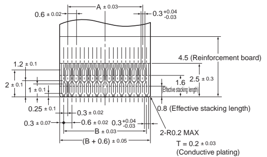
Applicable FPC Dimensions
