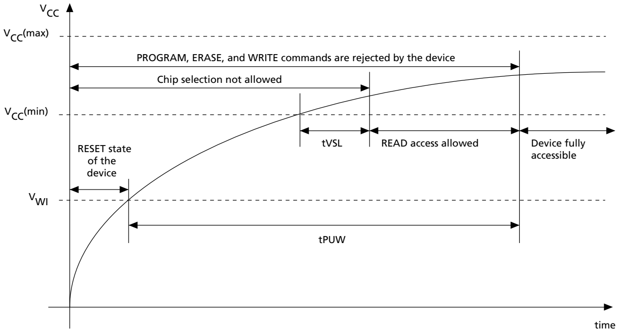
Figure 21: Power-Up Timing
