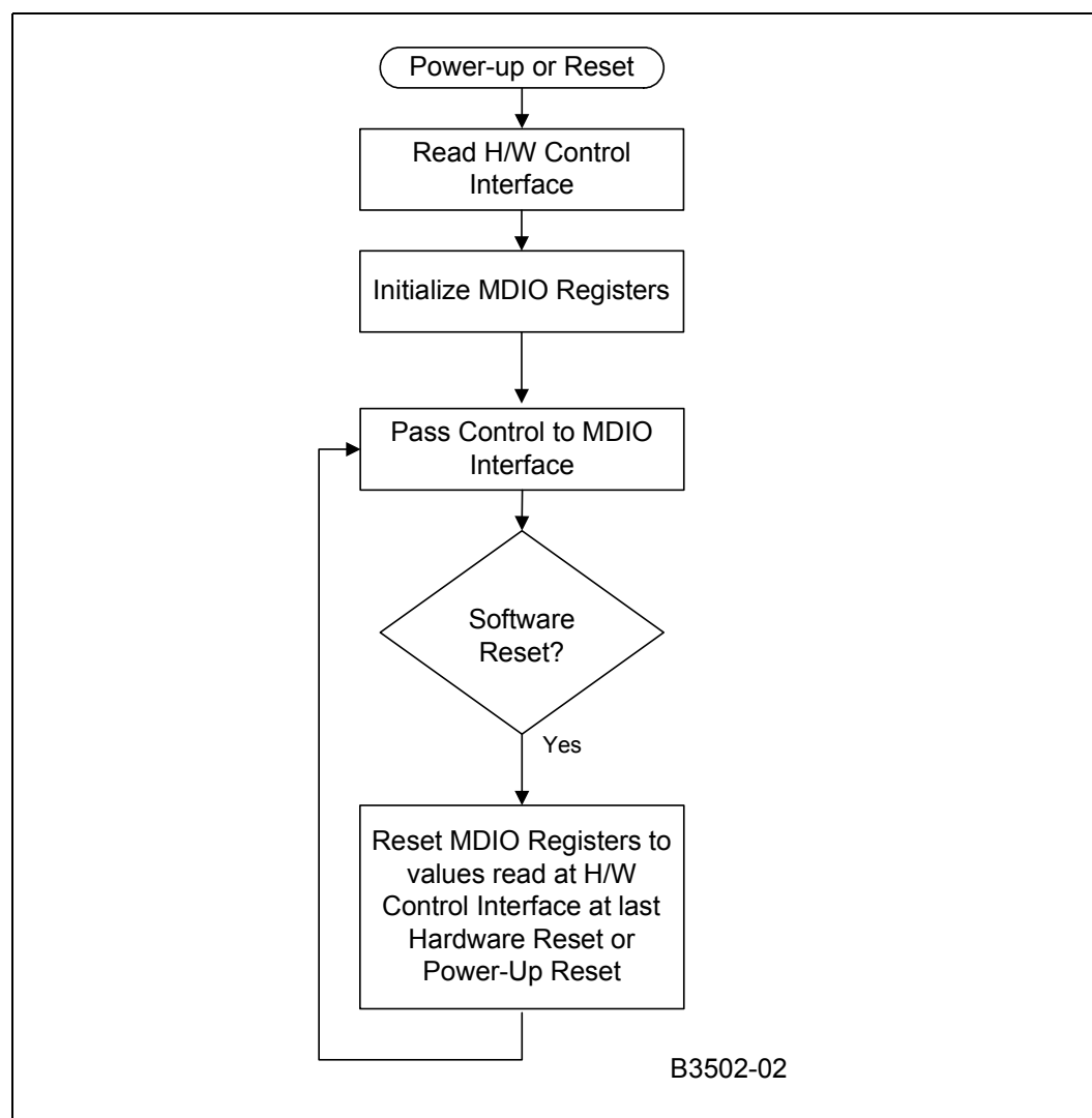
Figure 5 Initialization Sequence
