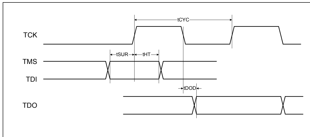
Figure 18 JTAG Timing
