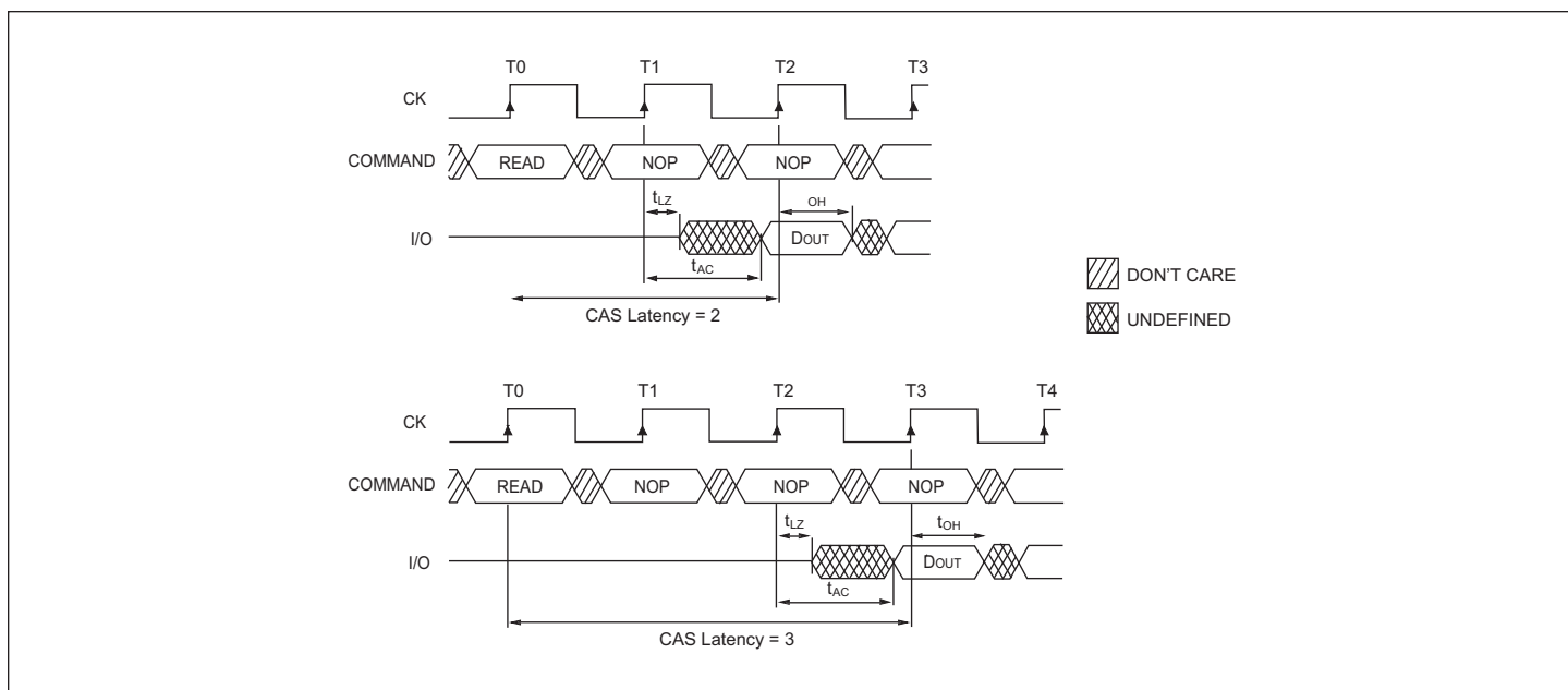
FIGURE 4 – CAS LATENCY
