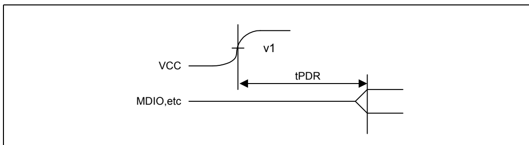
Figure 61 Power-Up Timing
