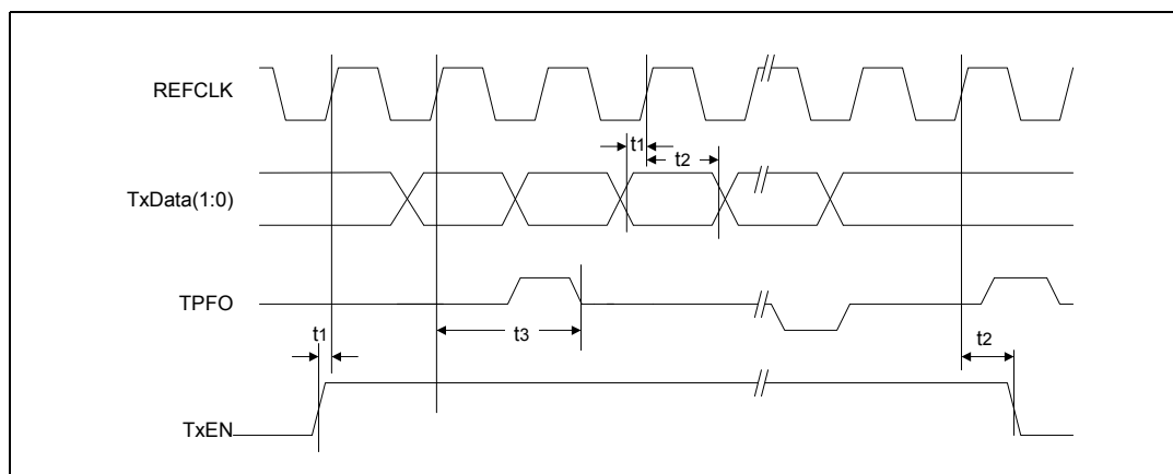
Figure 56 RMII - 10BASE-T Transmit Timing
