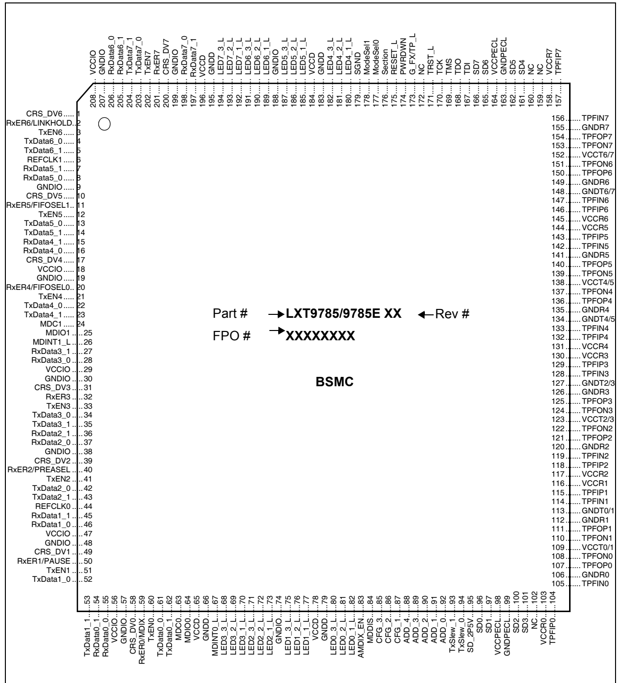
Figure 2 RMII 208-Pin PQFP Assignments
