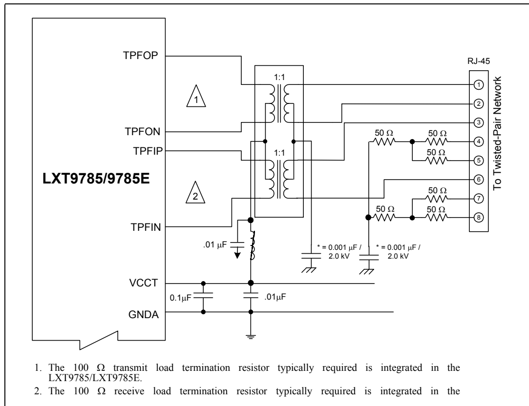
Figure 35 Typical Twisted-Pair Interface
