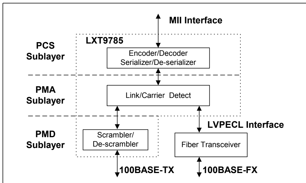
Figure 28 Protocol Sublayers
