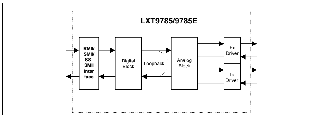
Figure 8 Internal Loopback
