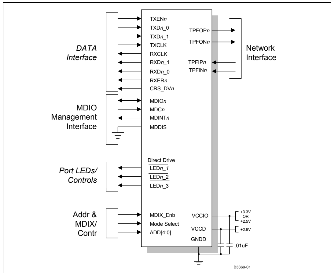
Figure 7 Interface Signals
