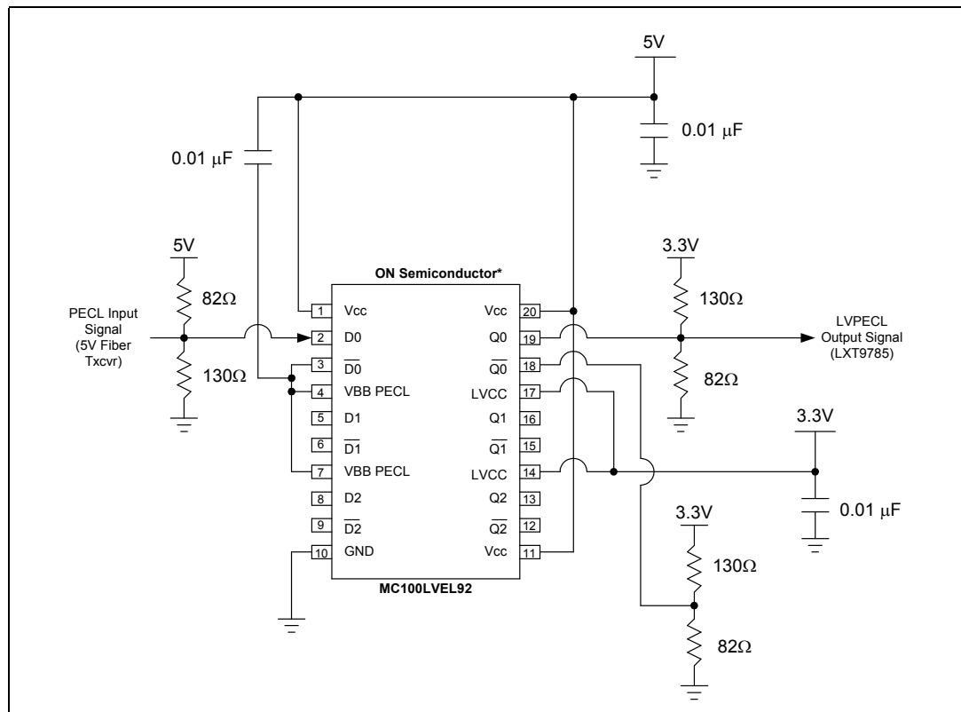
Figure 38 ON Semiconductor Triple PECL-to-LVPECL Translator
