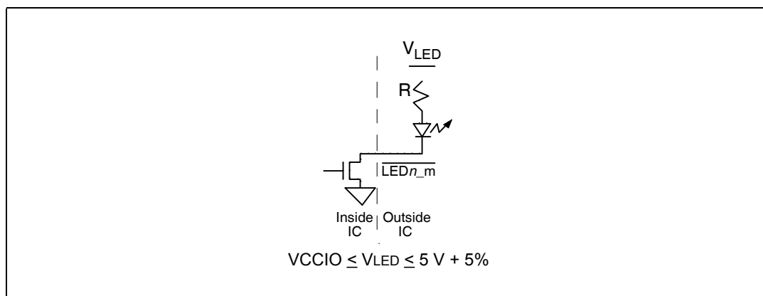
Figure 33 LED Circuit
