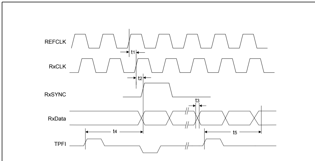
Figure 49 SS-SMII - 10BASE-T Receive Timing
