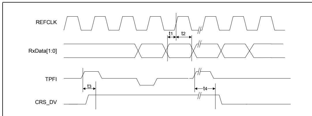
Figure 51 RMII - 100BASE-TX Receive Timing
