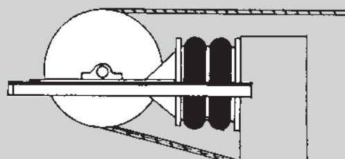
CABLE TENSIONING DEVICE
