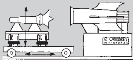
MISSILE ASSEMBLY FIXTURE
