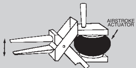
CORE STRAIGHTENER
