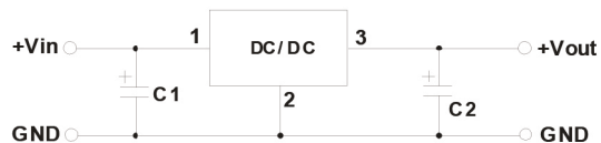
Positive output application circuit
