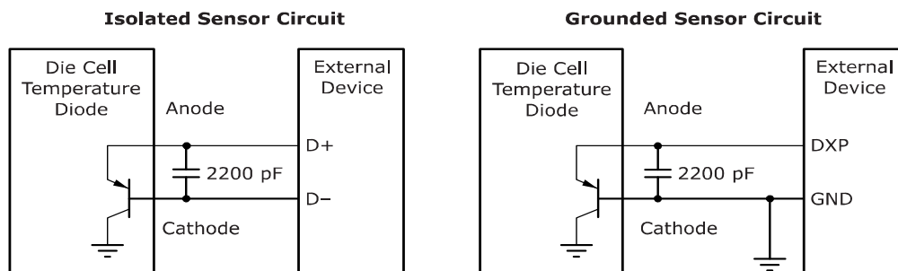
FIGURE 8-1: THERMAL DIODE
