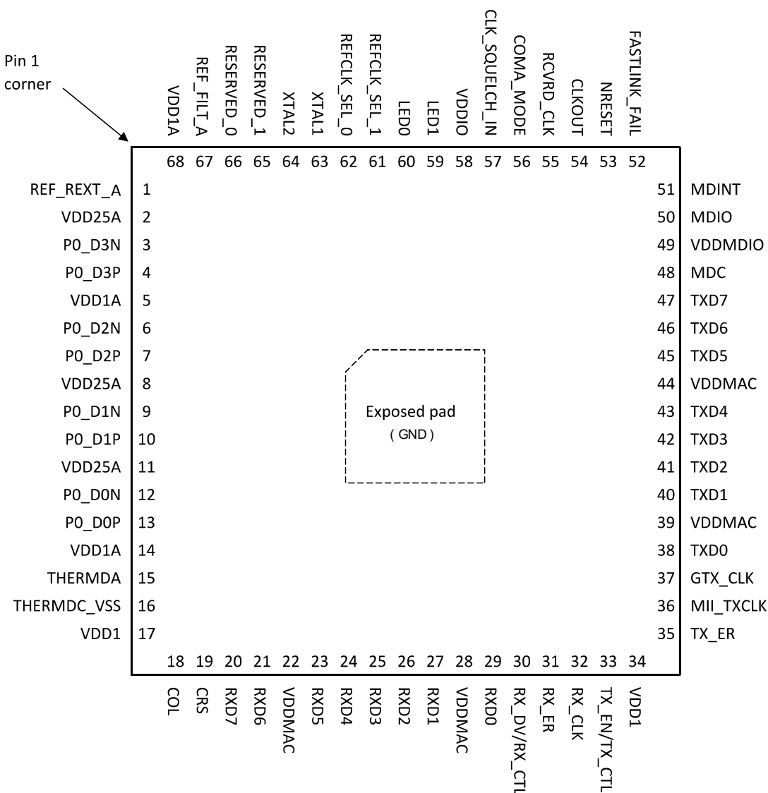
FIGURE 3-1: PIN DIAGRAM
