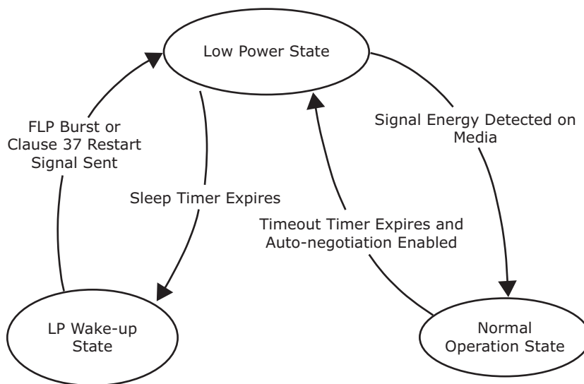
FIGURE 5-12: ACTIPHY STATE DIAGRAM
