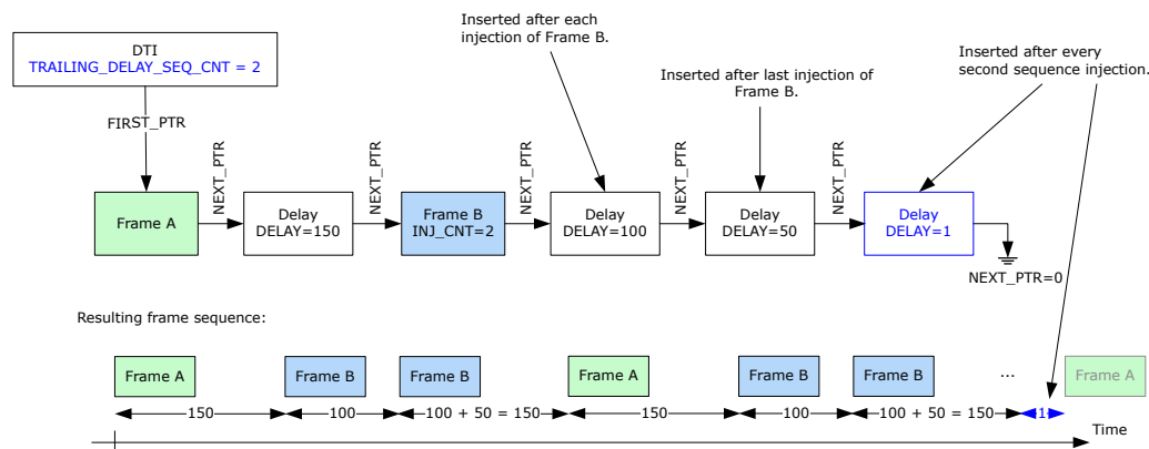
Figure 4-86. Fine Tuning Bandwidth of Multiframe DTI Sequence
