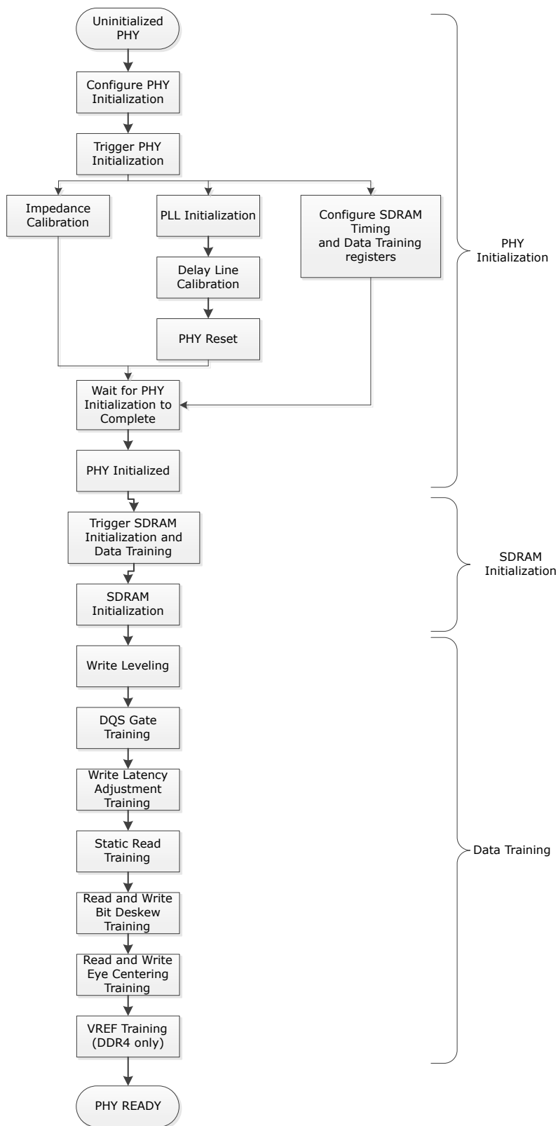
Figure 5-13. PHY Initialization Flow
