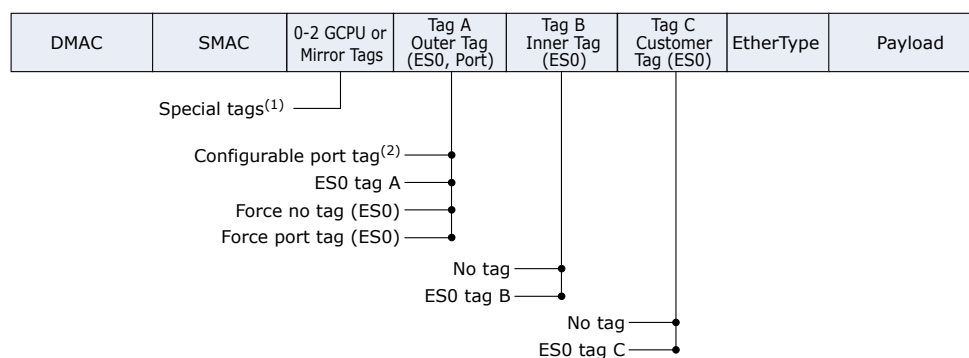
Figure 4-92. VLAN Pushing
