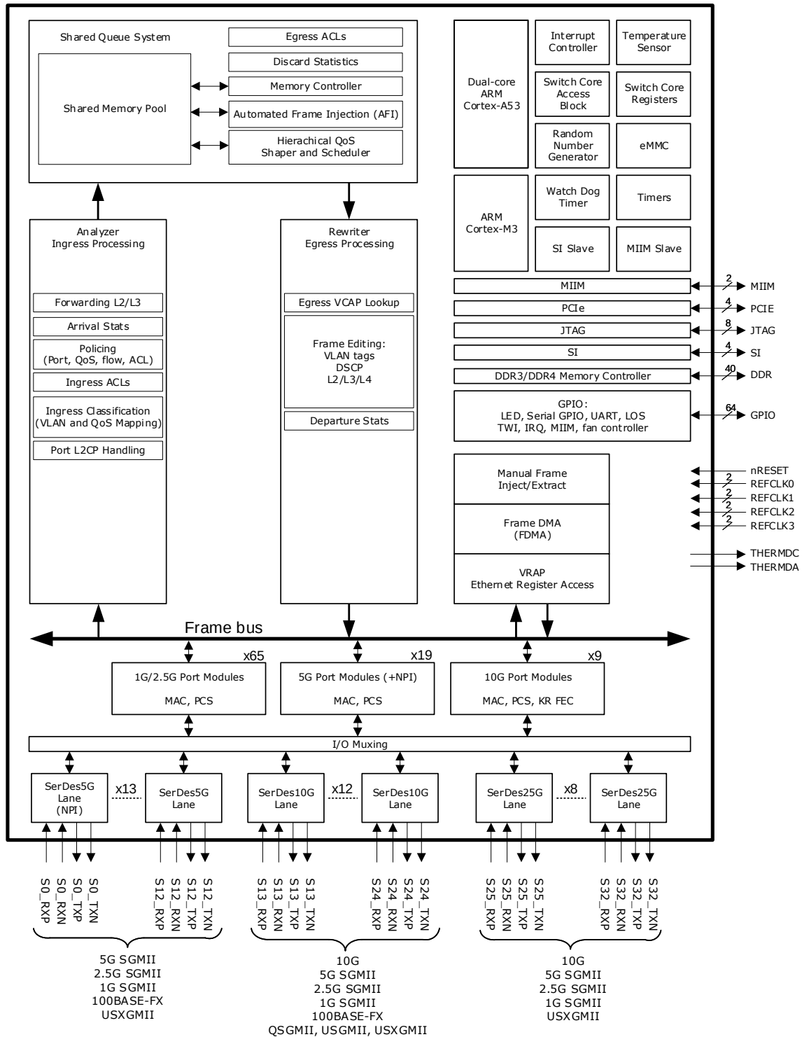
Figure 3-1. Block Diagram
