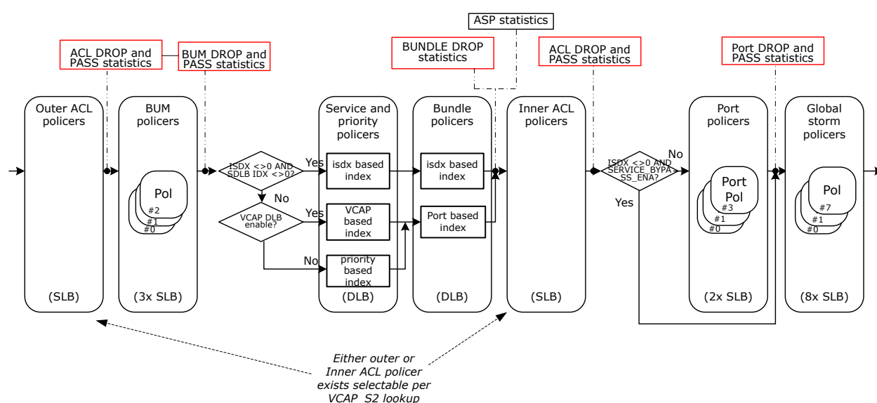
Figure 4-51. Policer Hierarchy
