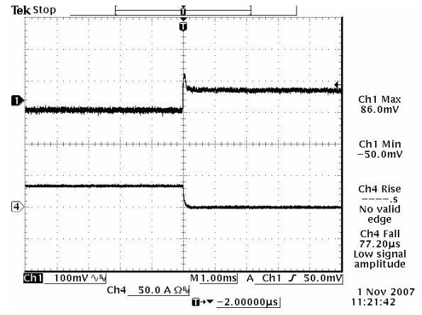
Vout=5 V 50%-0% Load Transients
