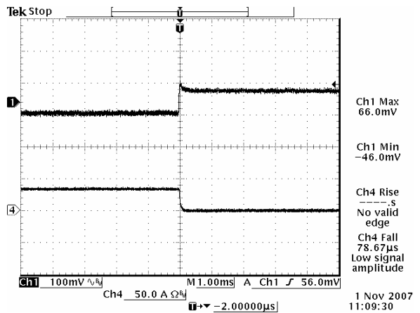
Vout=1.8 V 50%-0% Load Transients
