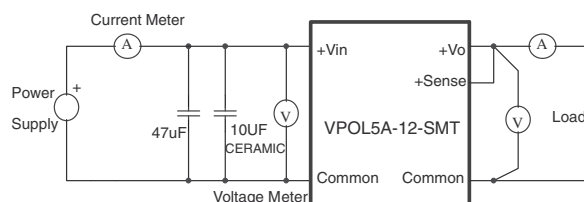
Figure 11. VPOL5A-12-SMT Test Setup
