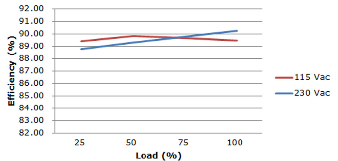
VOF-70B-24 Efficiency vs. Output Load (Natural Convection)
