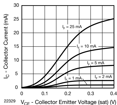
Fig. 8 - Collector Current vs. Collector Emitter Voltage (sat)
