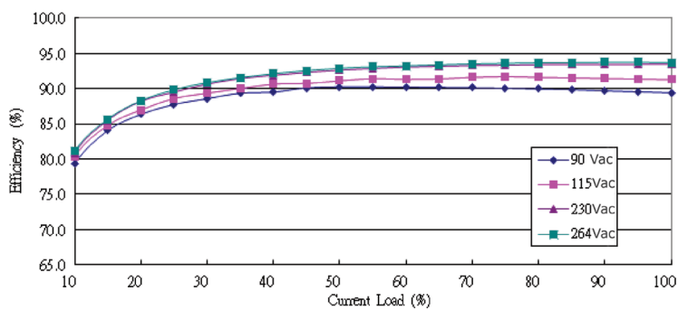
36 Vdc Output Efficiency Curve (at 25°C)
