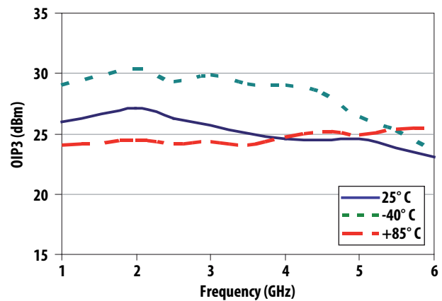
Figure 10. OIP3 Over Temp
