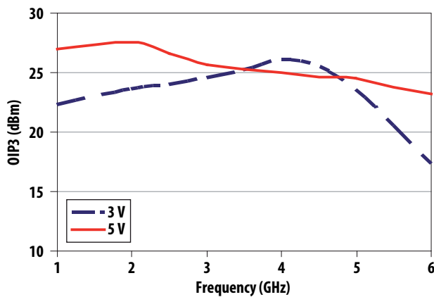
Figure 5. OIP3 Over Bias
