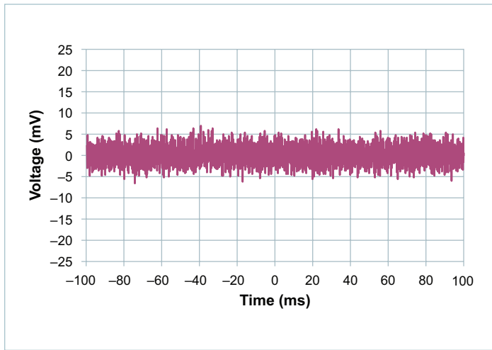
Figure 15 — VS3 (+5V) ripple with no load, AC-coupled
