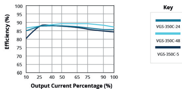
EFFICIENCY VS OUTPUT LOAD (VIN = 230 VAC)
