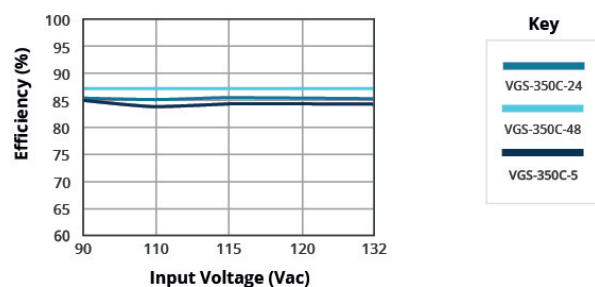
EFFICIENCY VS INPUT VOLTAGE (FULL LOAD)
