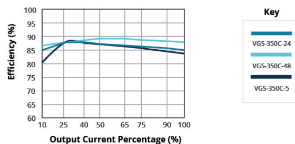
EFFICIENCY VS OUTPUT LOAD (VIN = 115 VAC)
