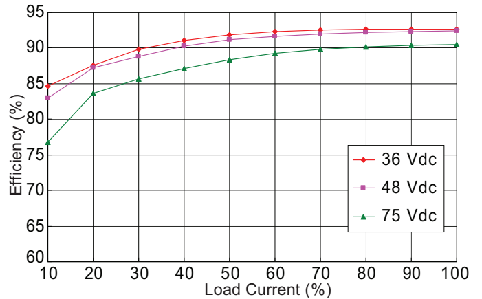
VFB600-D48-S32 Efficiency Curve (Efficiency vs. Line Voltage and Load Current)
