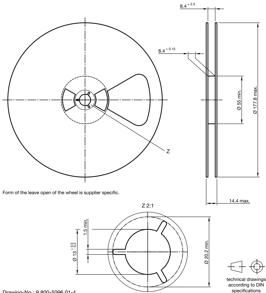
Fig. 8 - 7" Reel, 3000 Pieces
