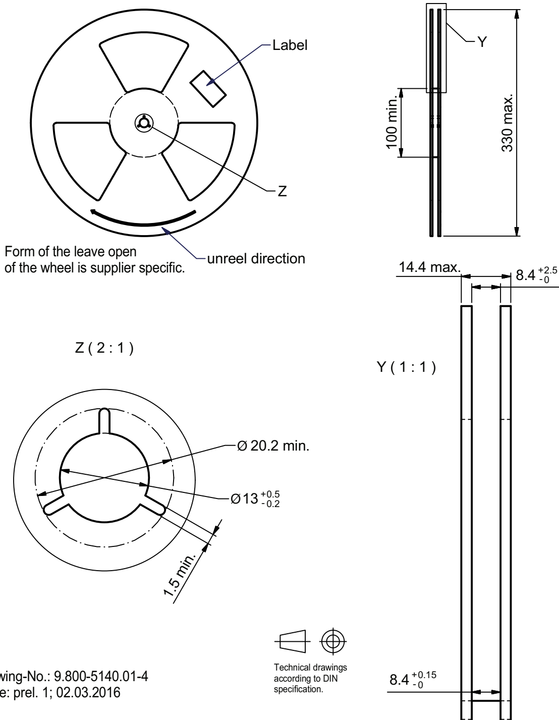
Fig. 9 - 13" Reel, 10 000 Pieces
