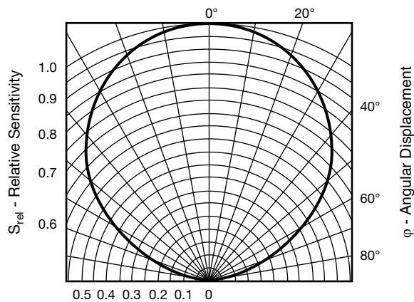
Fig. 4 - Relative Radiant Sensitivity vs. Angular Displacement
