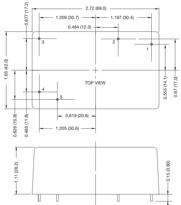
Encapsulated version (-E)
