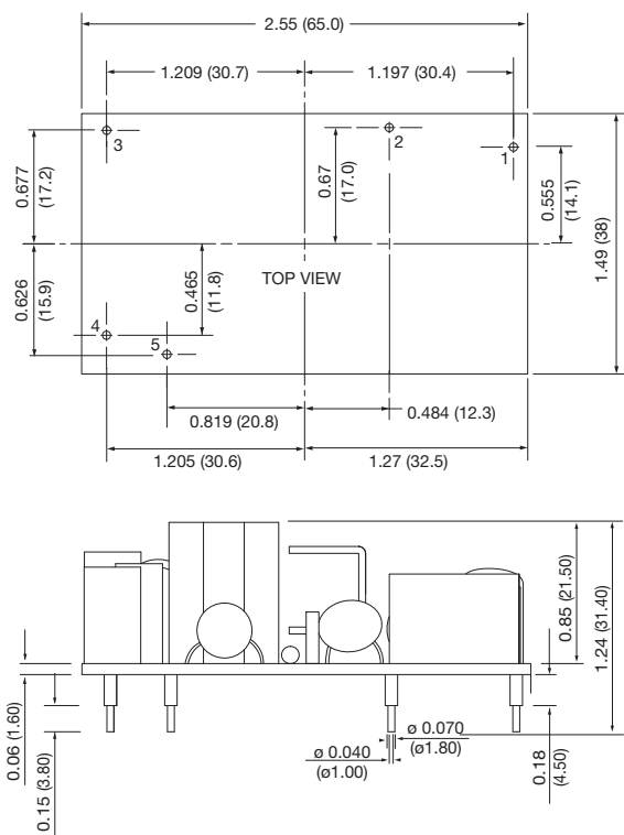
Open frame version
