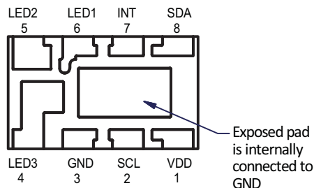
Pinning Bottom View
