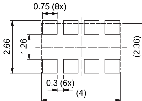
Recommended solder foot print
