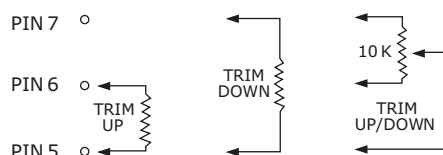
EXTERNAL OUTPUT TRIMMING
