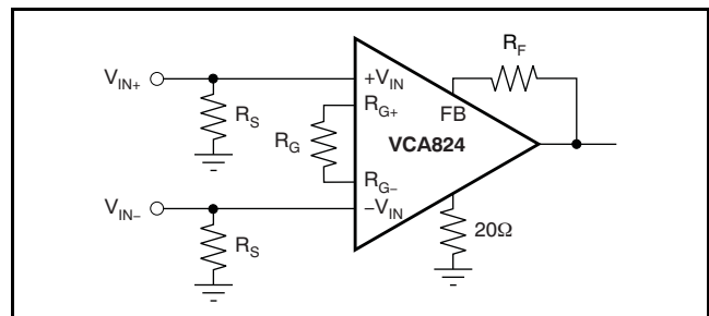
Figure 78. Difference Amplifier
